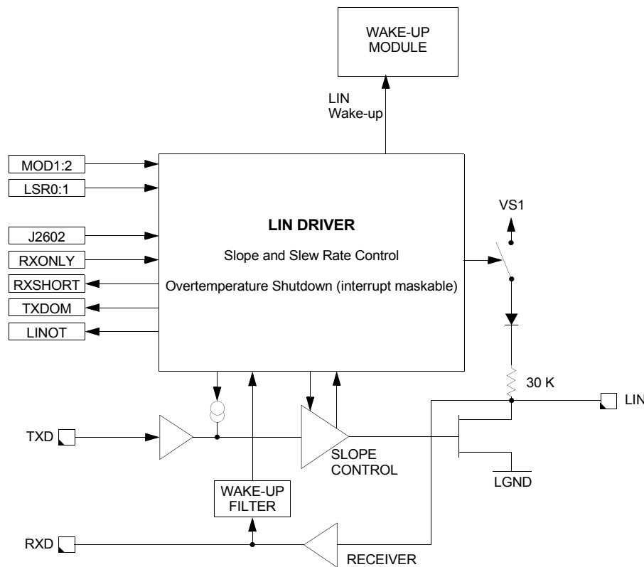
Figure 18. LIN interface
