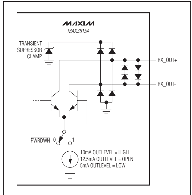
Figure 6. Simplified Output Circuit Schematic
