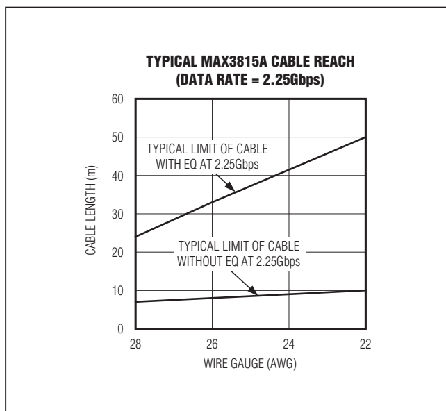
Figure 7. Cable Reach
