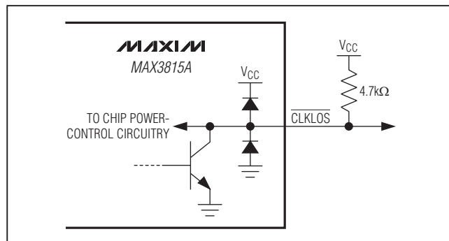
Figure 3. Simplified \overline{\text{CLKLOS}} Output Circuit Schematic
