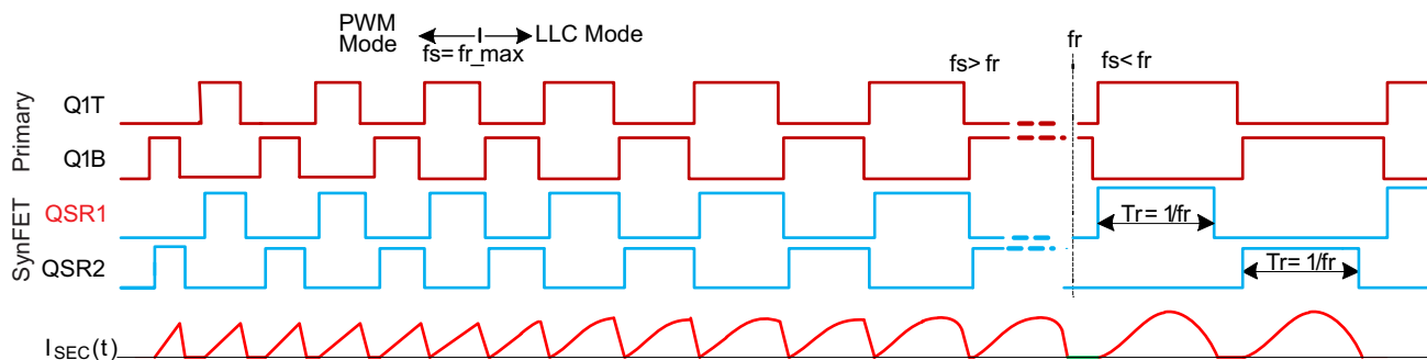
Figure 6-6. LLC Waveforms
