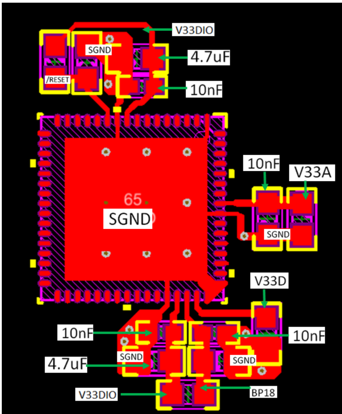
Figure 7-13. Layout Example
