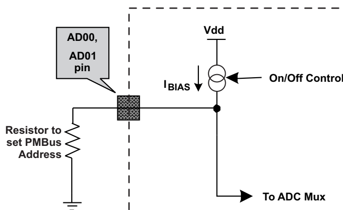
Figure 6-17. PMBUS Address Detection Method
