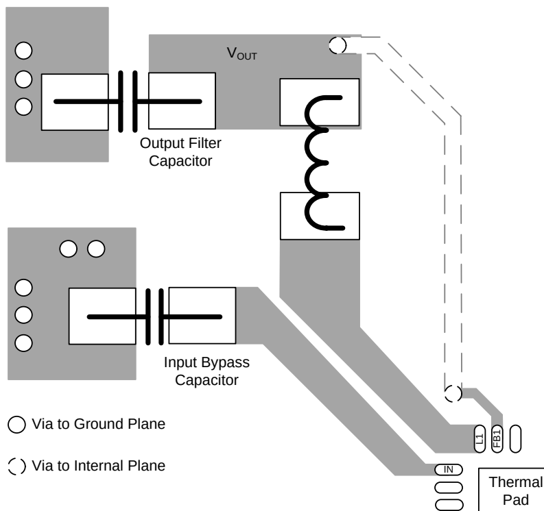
Figure 8-1. Layout Recommendation
