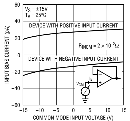
Input Bias Current vs Common Mode Range
