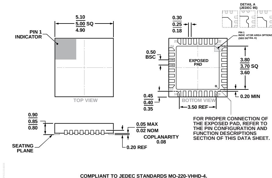
Figure 18. 32-Lead Lead Frame Chip Scale Package [LFCSP] 5 mm × 5 mm Body and 0.85 mm Package Height (HCP-32-1)
