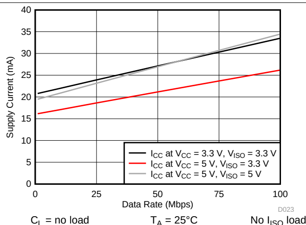
Figure 12. ISOW7840 Supply Current vs Data Rate
