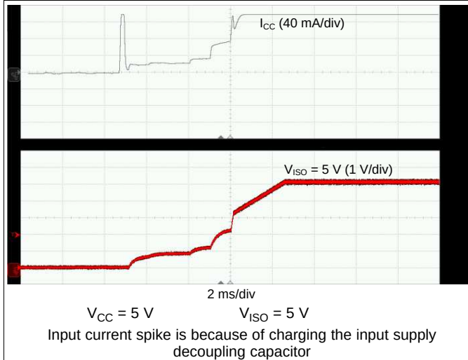
Figure 29. Soft Start at 130-mA Load
