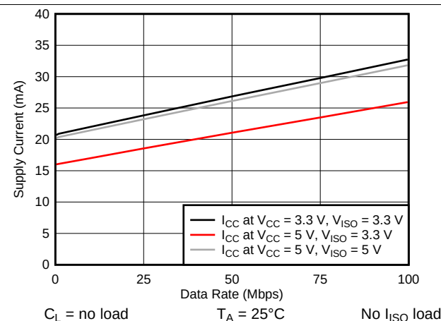
Figure 14. ISOW7841 Supply Current vs Data Rate
