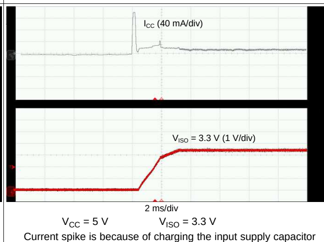
Figure 26. Soft Start at 10-mA Load
