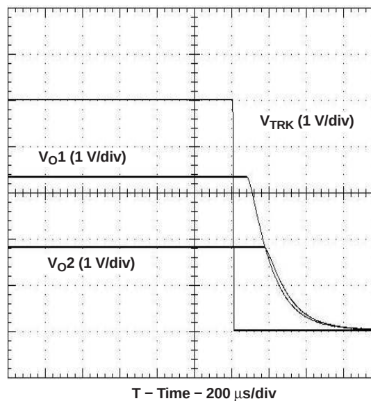
Figure 29. Simultaneous Power Down With Auto-Track Control
