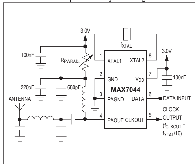
Figure 1. Output Power Adjustment Circuit
