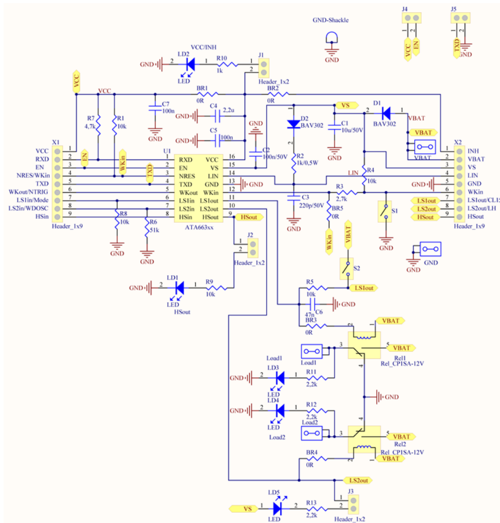
Figure 5-1. Board Schematic
