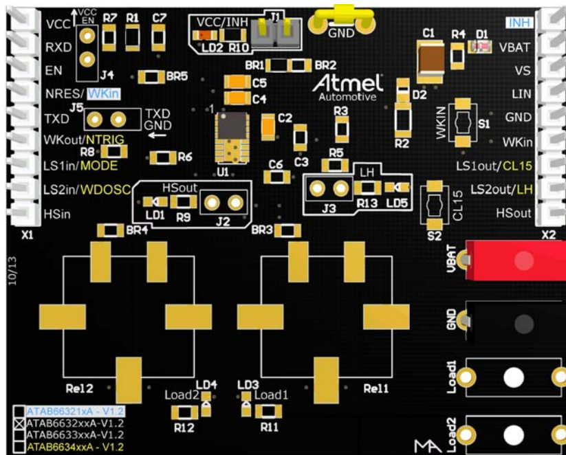
Figure 7-1. Atmel ATA663201 and ATA663203 (Voltage Regulator)
