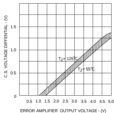
Figure 4 • Current Sense Threshold Vs. Error Amplifier Output
