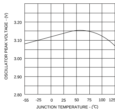
Figure 7 • Oscillator Peak Voltage Vs. Temperature
