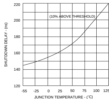
Figure 10 • Shutdown Delay To Output Vs. Temperature
