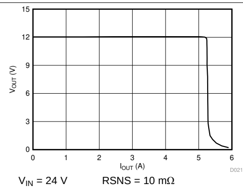
Figure 20. Constant Current Constant Voltage (CCCV) Operation
