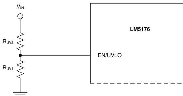
Figure 22. UVLO Threshold Programming
