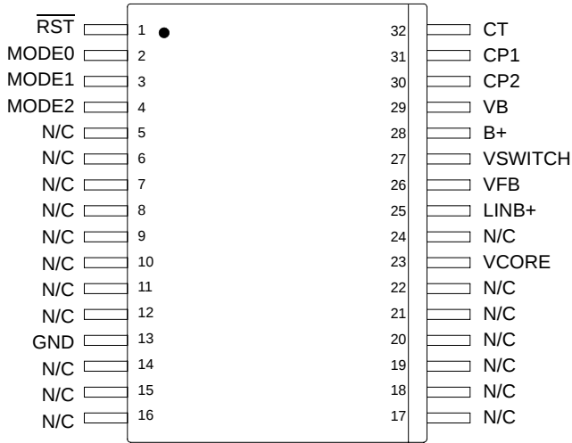
Figure 3. 34710 Pin Connections
