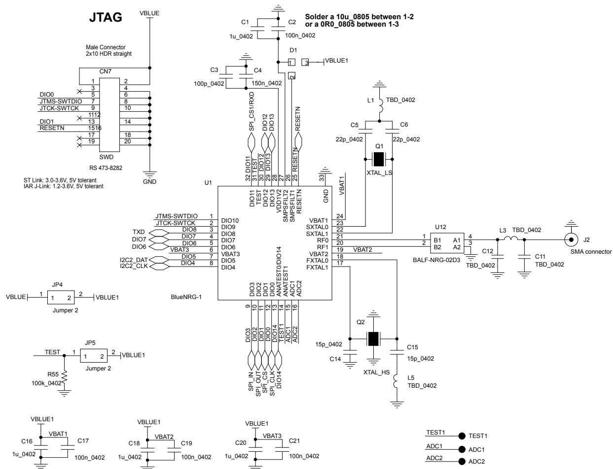
Figure 43. STEVAL-IDB007V2 - scheme 1
