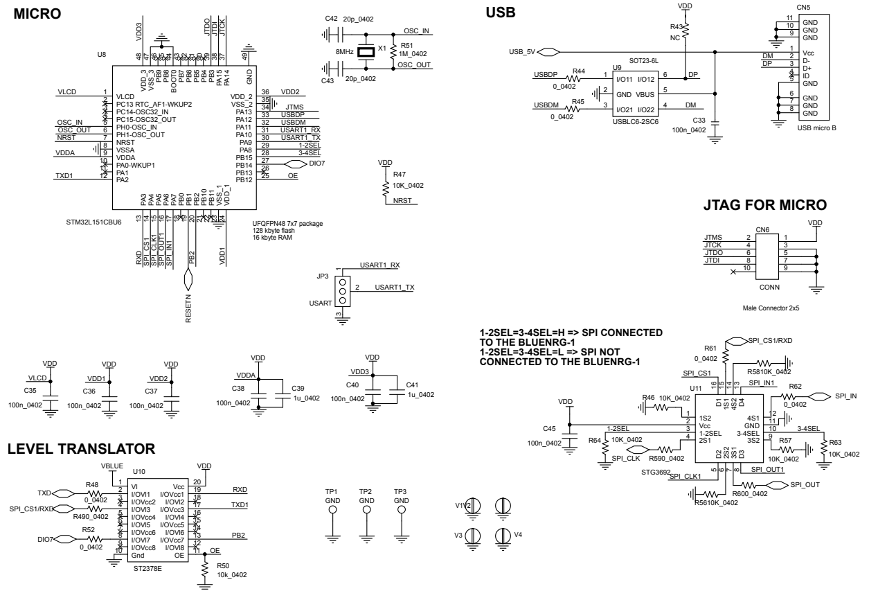
Figure 44. STEVAL-IDB007V2 - scheme 2
