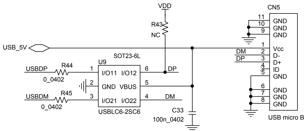
Figure 53. STEVAL-IDB008V2 - USB
