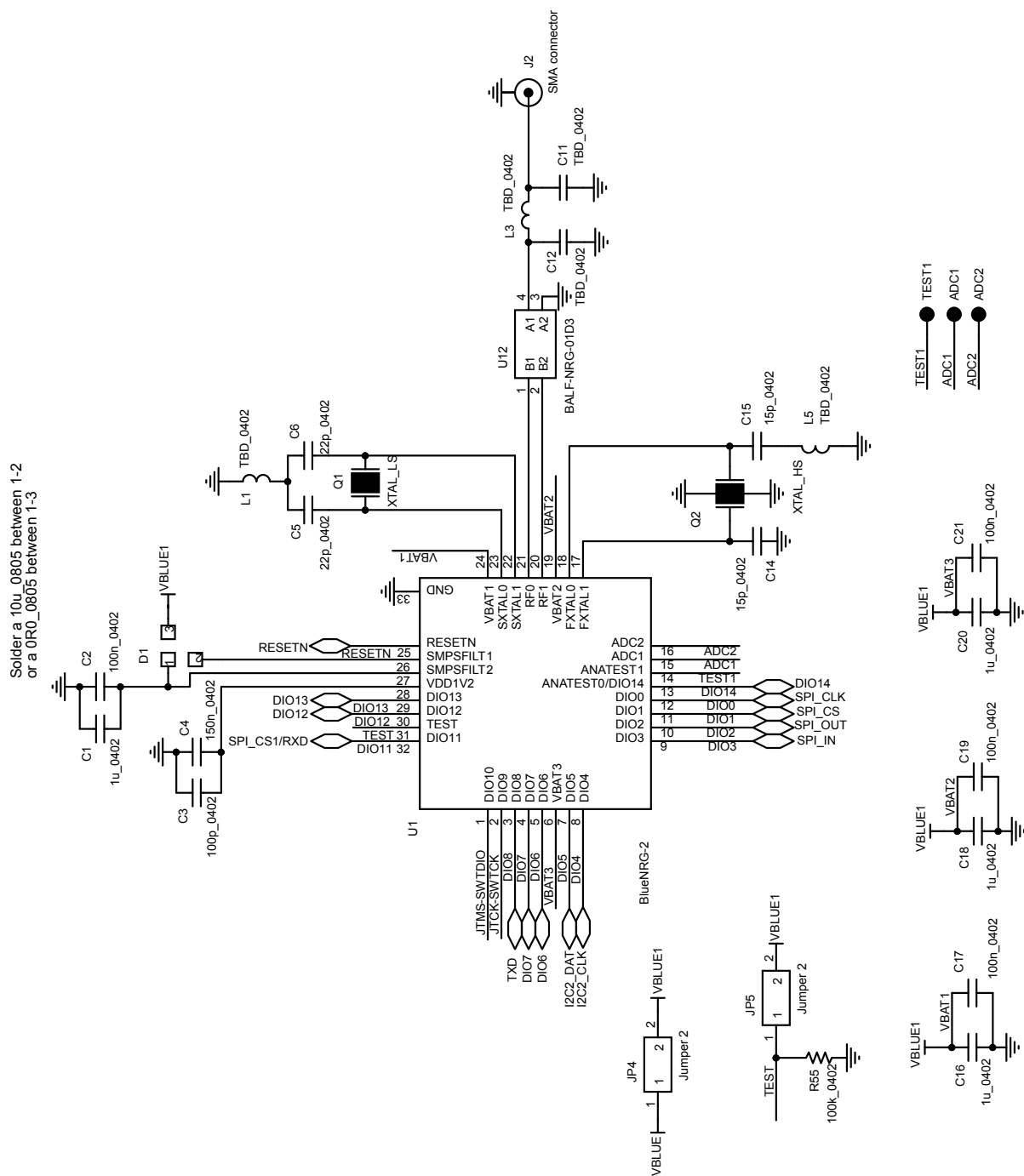
Figure 33. STEVAL-IDB008V1 BlueNRG-2
