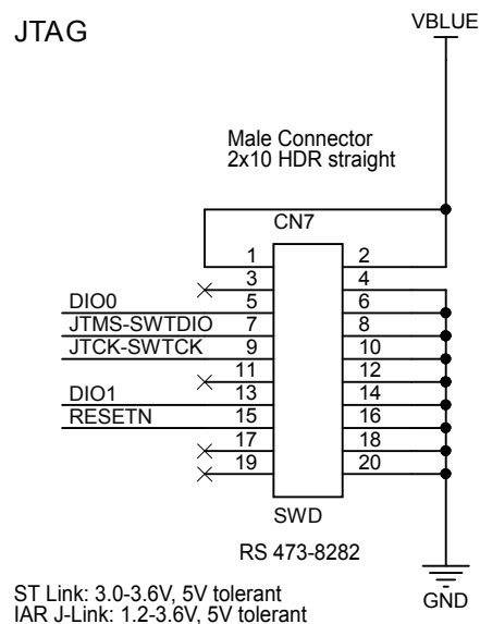
Figure 24. STEVAL-IDB007V1 JTAG
