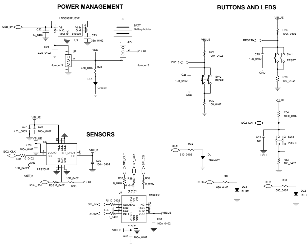
Figure 45. STEVAL-IDB007V2 - scheme 3
