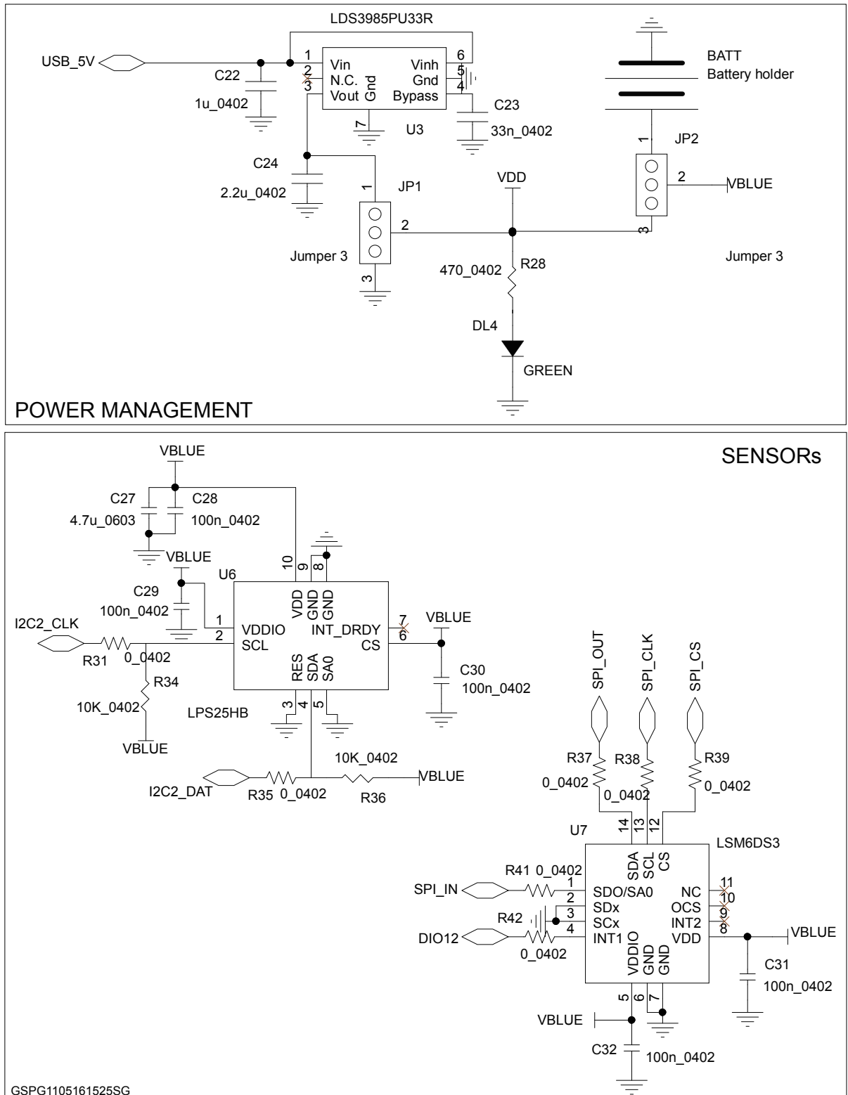
Figure 26. STEVAL-IDB007V1 power management, sensors
