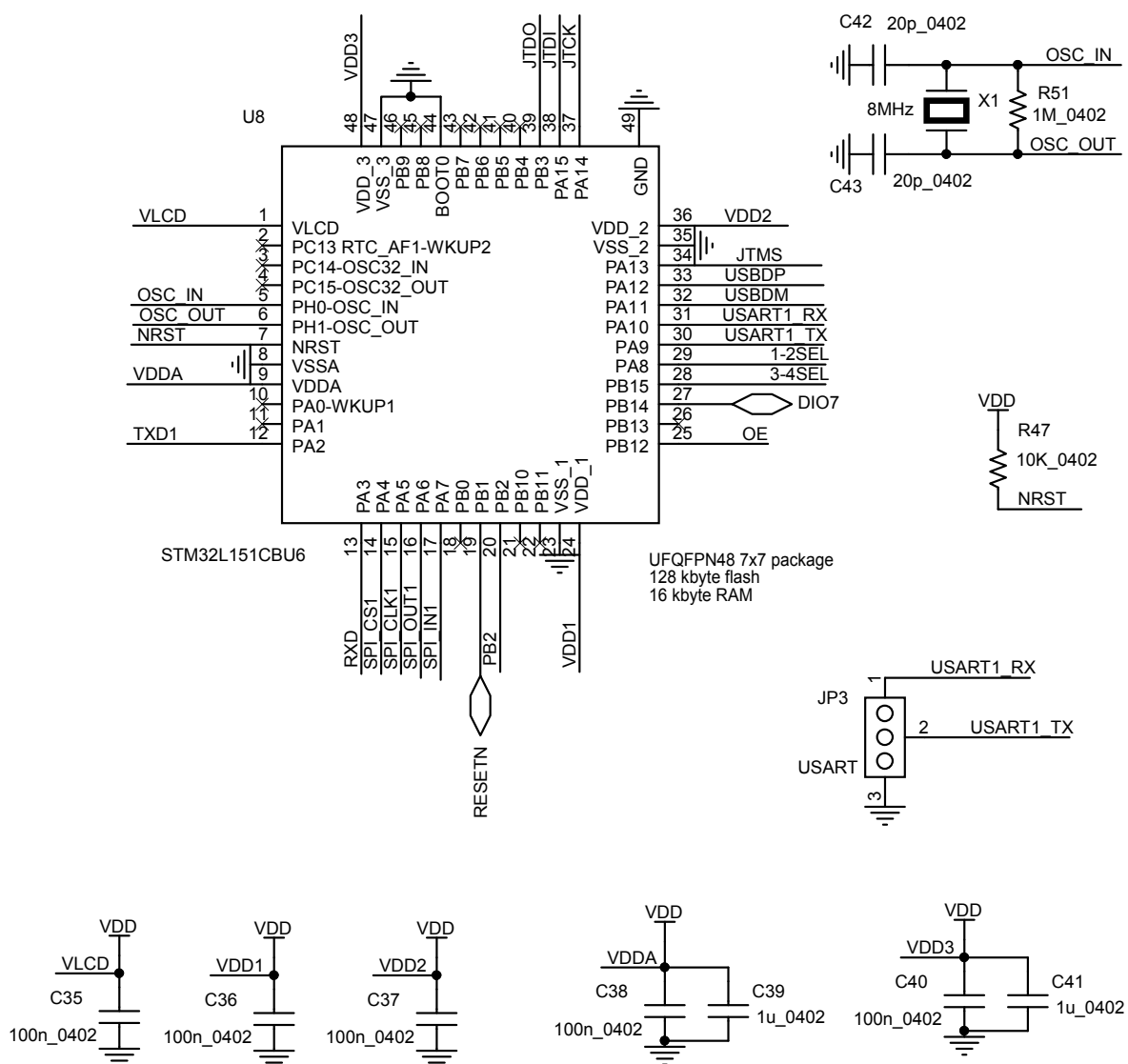
Figure 52. STEVAL-IDB008V2 - micro
