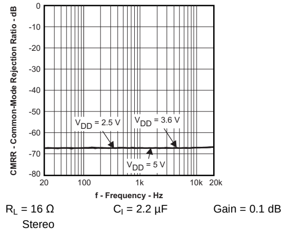
Figure 26. Common Mode Rejection Ratio vs Frequency
