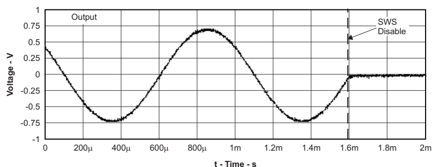
Figure 46. Shutdown Time
