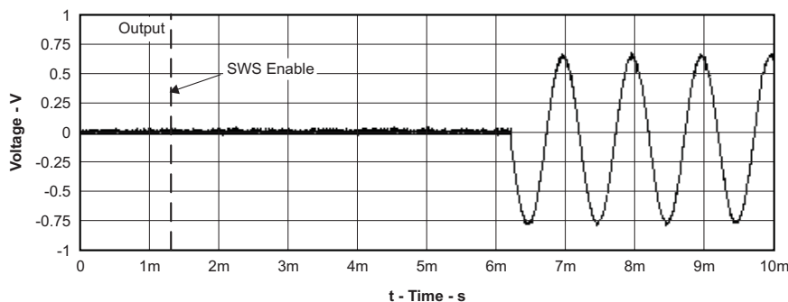
Figure 47. Startup Time
