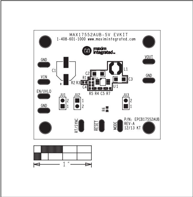
Figure 2. MAX17552 5V EV Kit (μMAX) Component Placement Guide—Component Side
