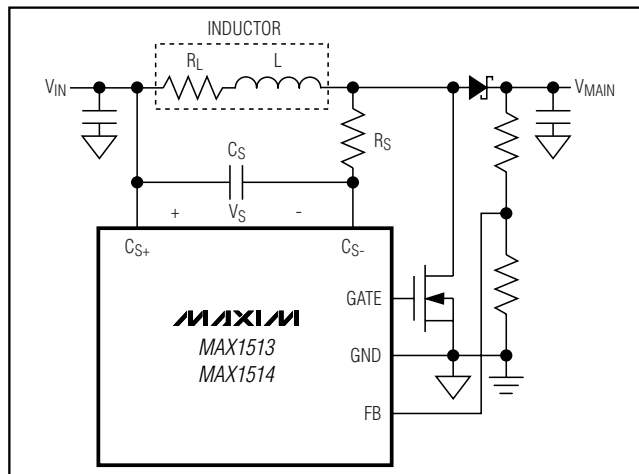
Figure 5. Step-Up Regulator Using Lossless Current Sensing
