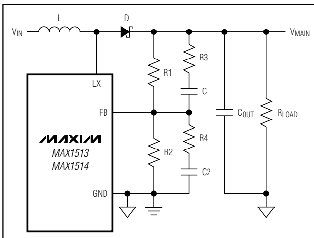
Figure 11. Feedback Compensation
