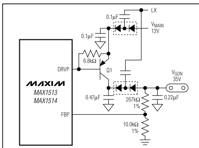
Figure 7. Linear Regulator Controls Intermediate Charge-Pump Stage
