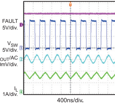
Steady State I_{LED} = 1.5A
