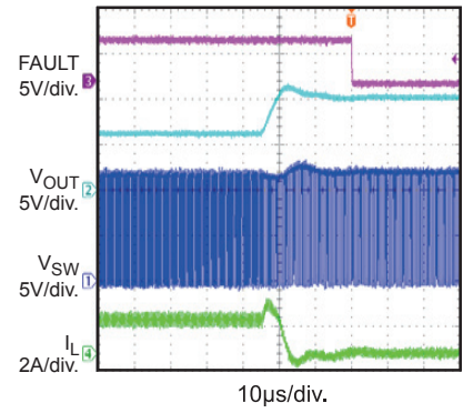
LED Open Entry
