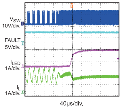
LED+ and LED- Short Recovery
