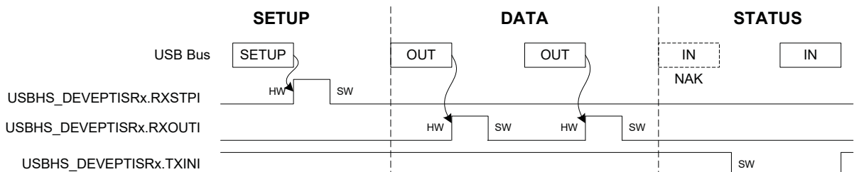
Figure 39-9. Control Write
