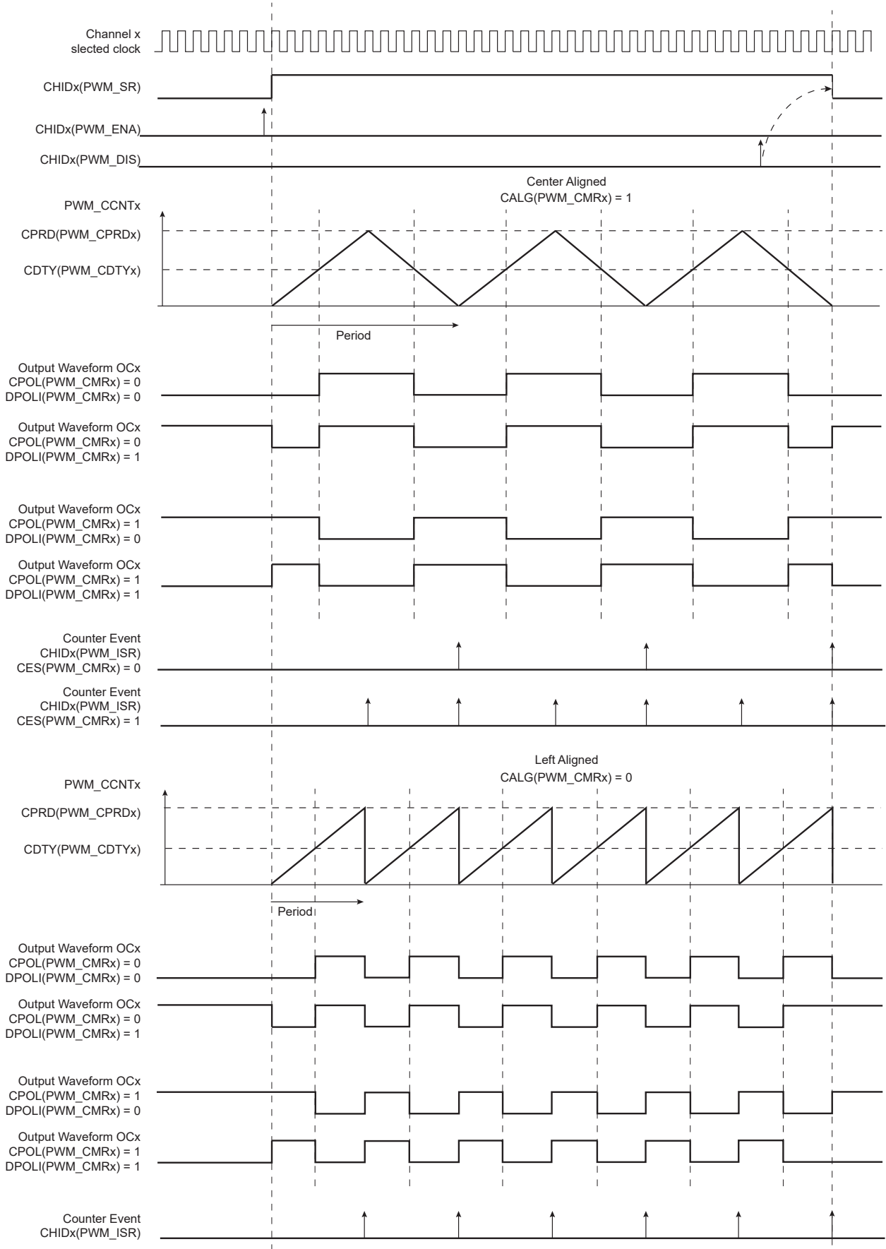
Figure 51-5. Waveform Properties
