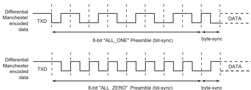
Figure 46-57. Preamble Patterns
