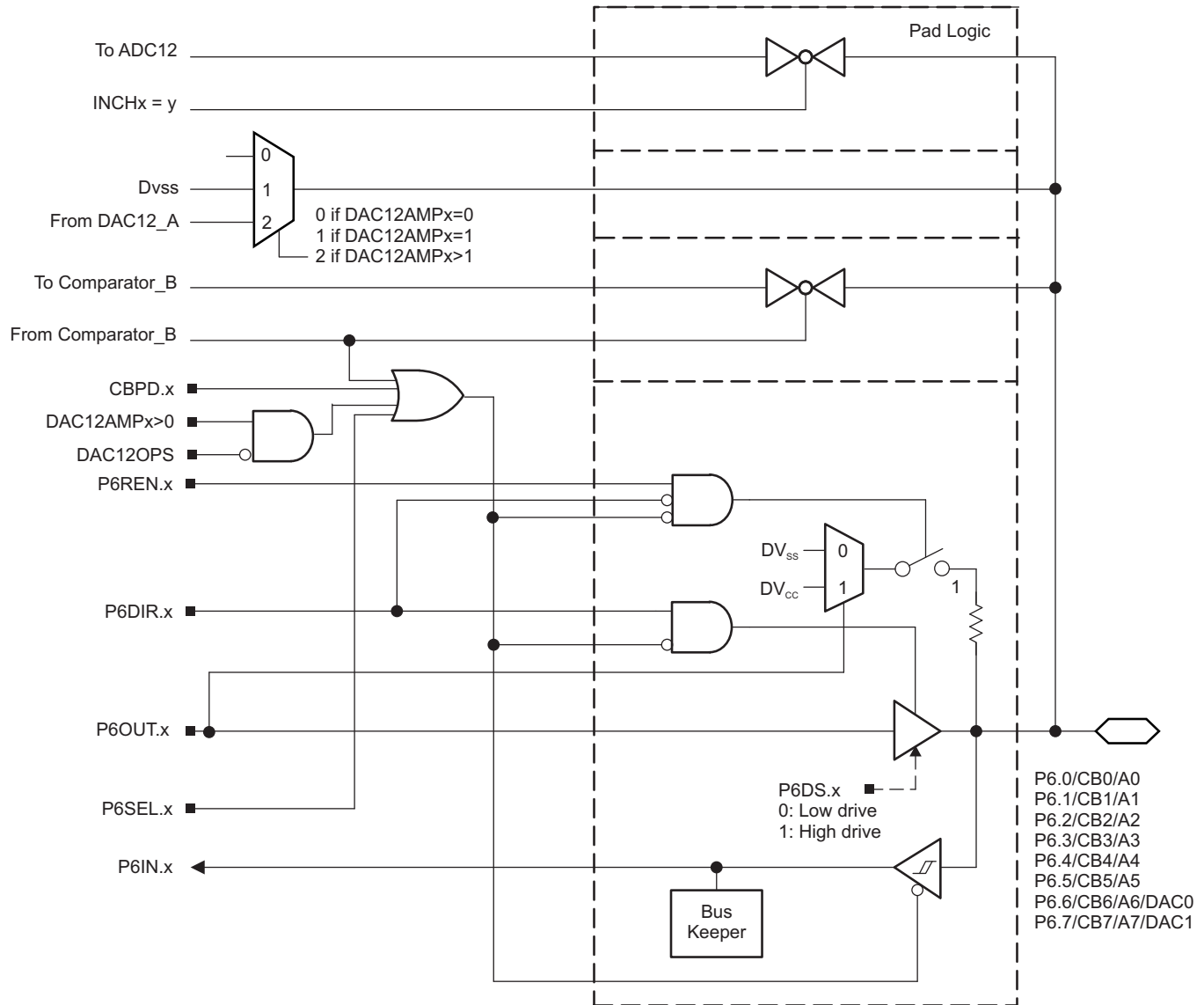
Figure 6-8. Port P6 (P6.0 to P6.7) Diagram
