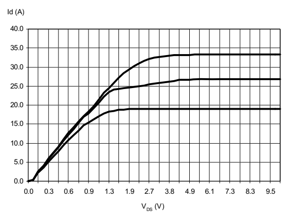
Figure 23. Output characteristics
