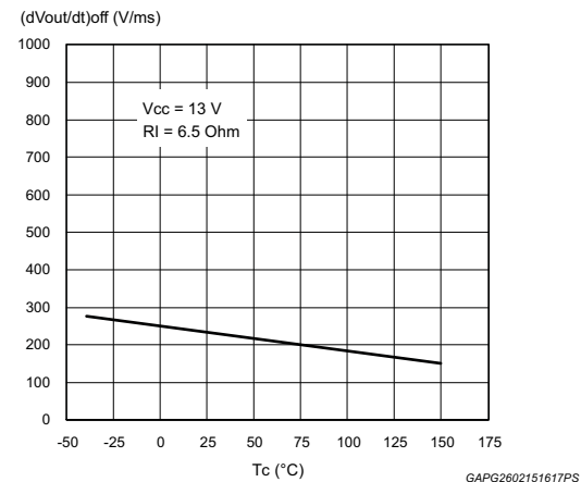
Figure 17. Turn-off voltage slope
