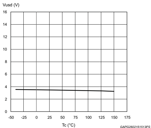
Figure 14. Undervoltage shutdown
