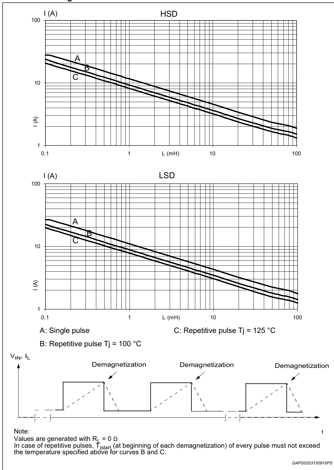
Figure 29. Maximum turn-off current vs load inductance
