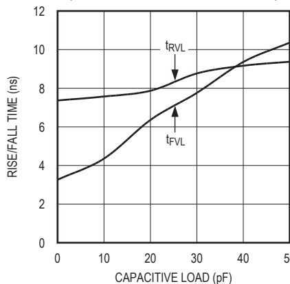
RISE/FALL TIME vs. CAPACITIVE LOAD (PUSH-PULL DRIVING ONE I/O V_{CC} )
