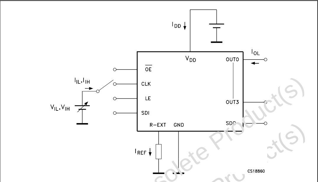
Figure 11. DC characteristic
