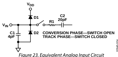
Figure 23. Equivalent Analog Input Circuit
