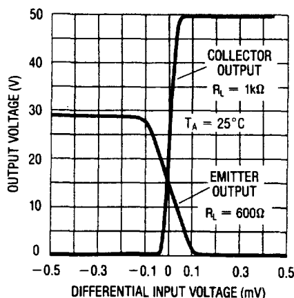
Transfer Function
