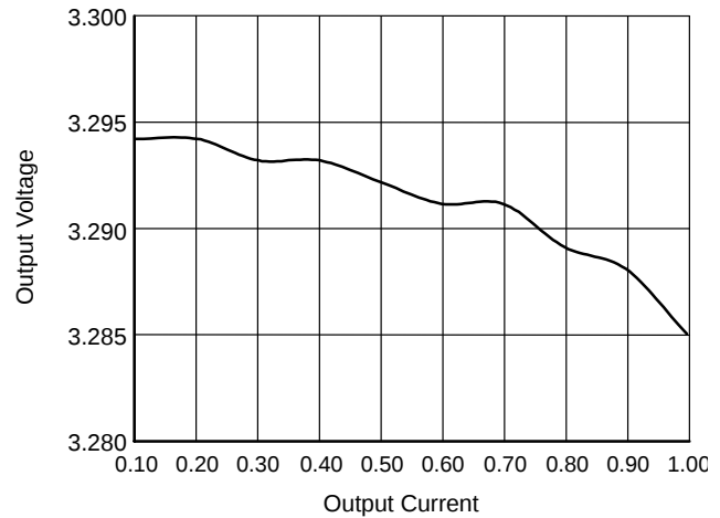
Figure 4. Load Regulation
