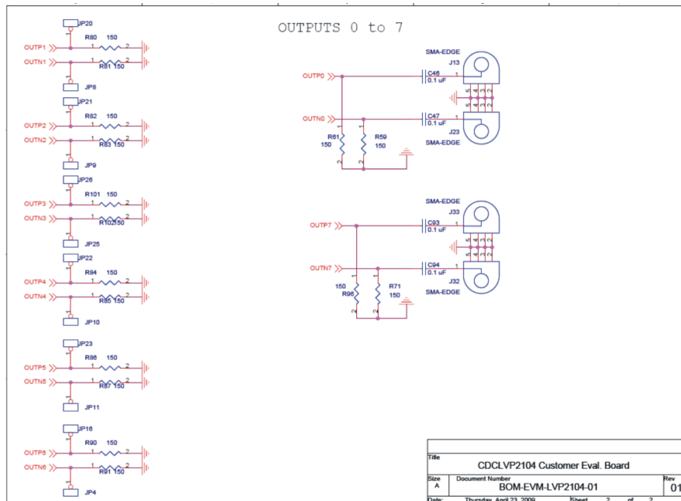
Figure 3. CDCLVP2104EVM—Schematic
