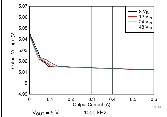
Figure 23. Load Regulation
