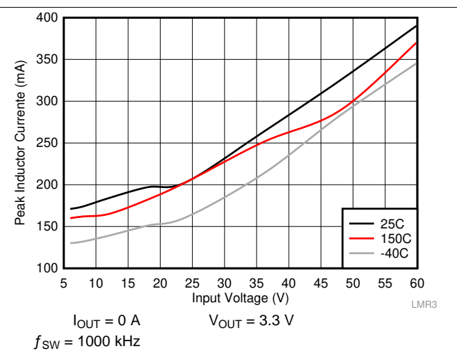
Figure 6. I PEAK-MIN
