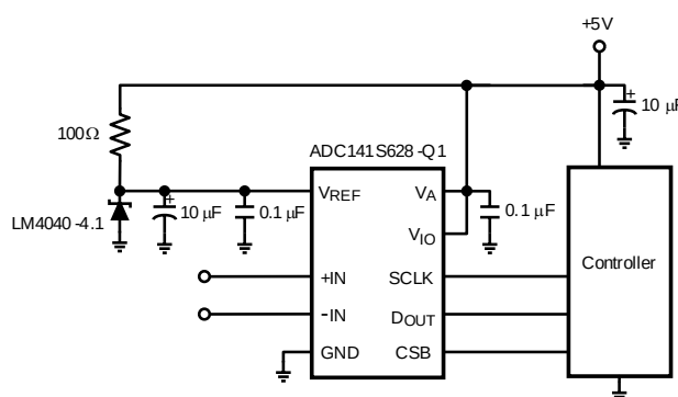
Figure 35. Low-Cost, Low-Power Data Acquisition System
