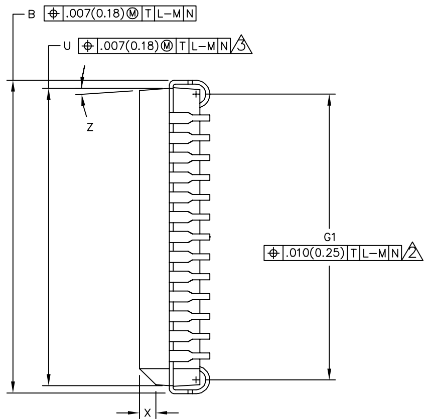
VIEW D-D
