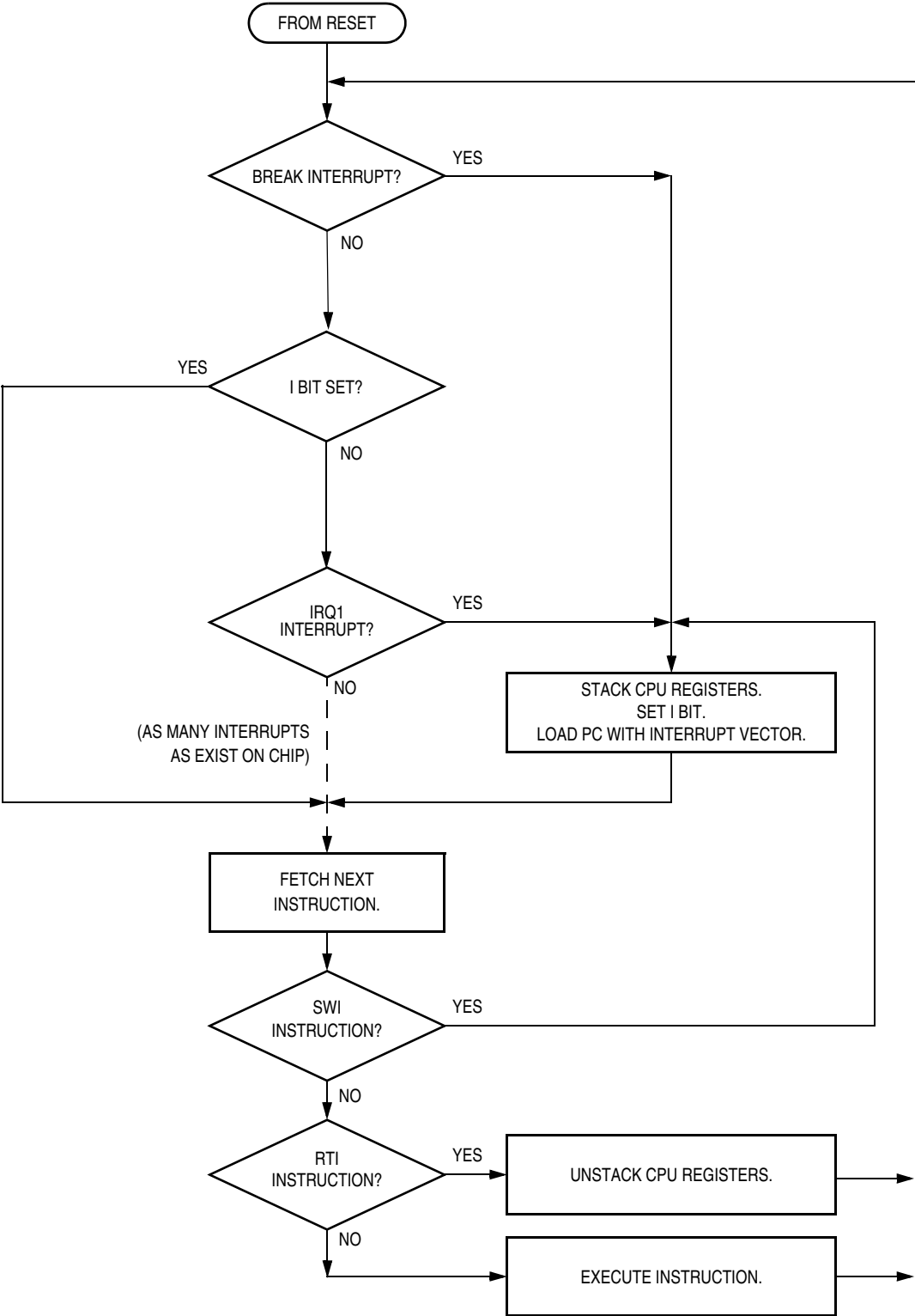
Figure 15-9. Interrupt Processing
