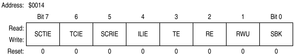
Figure 14-10. SCI Control Register 2 (SCC2)
