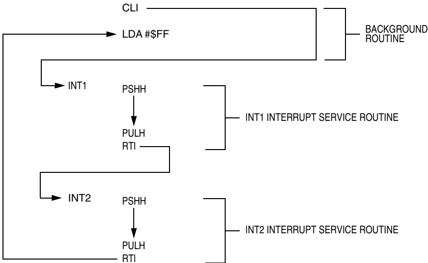
Figure 15-11. Interrupt Recognition Example
