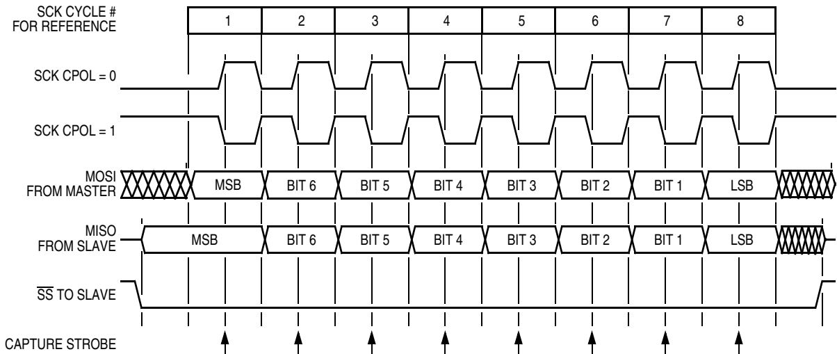
Figure 16-4. Transmission Format (CPHA = 0)
