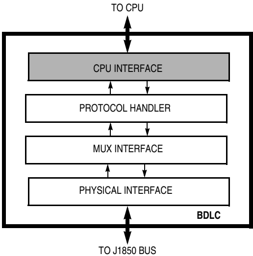
Figure 4-15. BDLC Block Diagram
