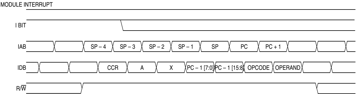
Figure 15-10. Interrupt Recovery
