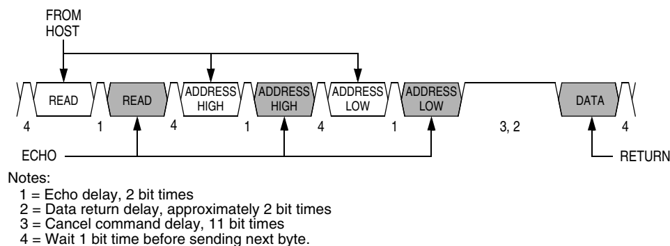
Figure 18-10. Read Transaction
