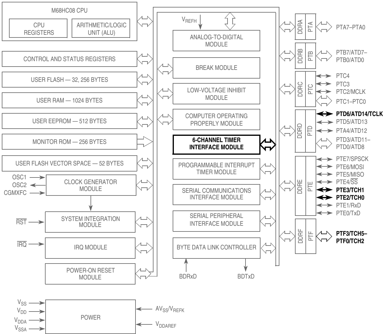
Figure 17-1. Block Diagram Highlighting TIM Block and Pins
