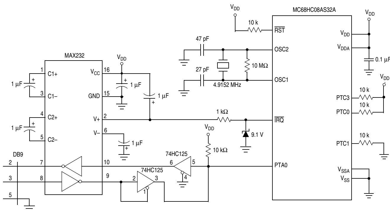
Figure 18-6. Normal Monitor Mode Circuit
