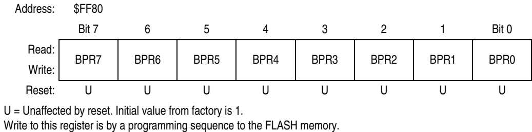
Figure 2-12. FLASH Block Protect Register (FLBPR)
