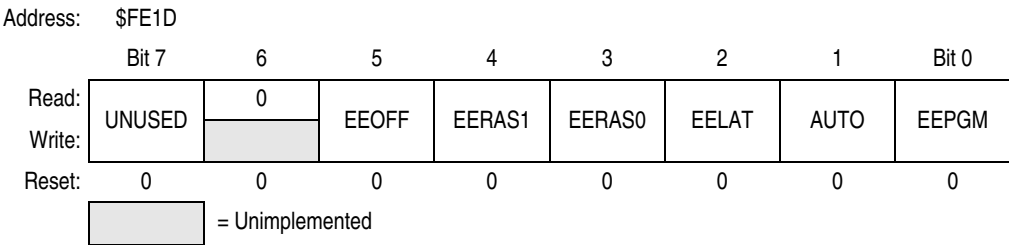
Figure 2-4. EEPROM Control Register (EECR)
