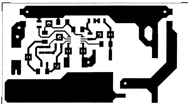
Figure 8. Top (Component) Layer as viewed from Top
