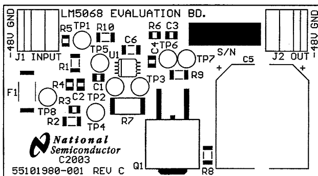
Figure 6. Silkscreen Layer as viewed from Top
