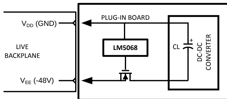
Figure 1. Live System Backplanes
