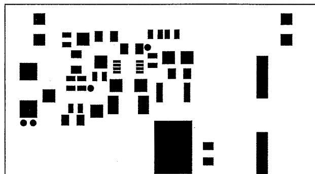
Figure 7. Top Side Soldermask as viewed from Top
