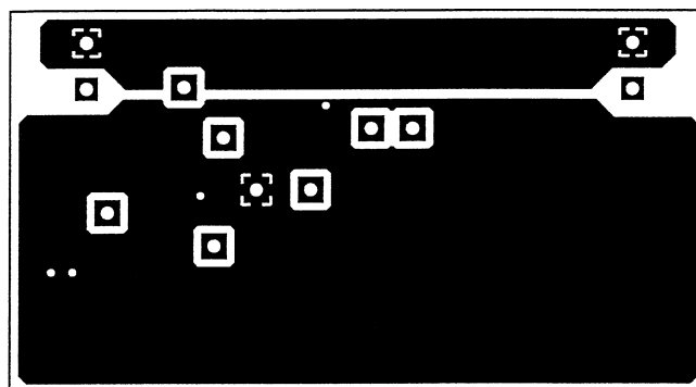
Figure 10. Bottom (Solder) Layer as viewed from Top
