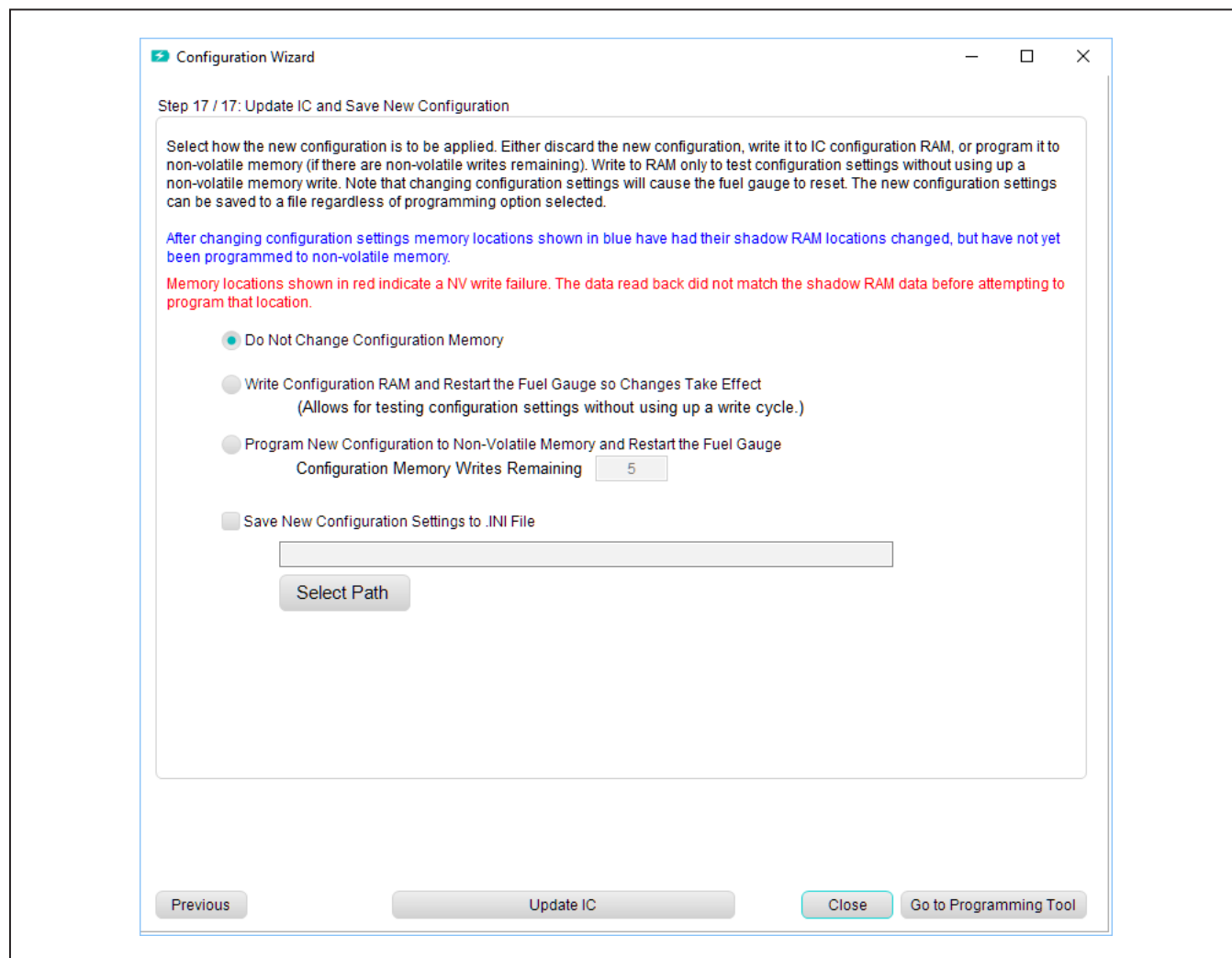
Figure 17. Configuration Step
