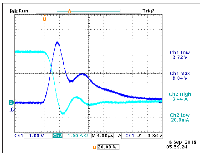
Figure 22. BATT Voltage and Battery Current Waveform at Overcurrent Protection Event with Bad Connections
