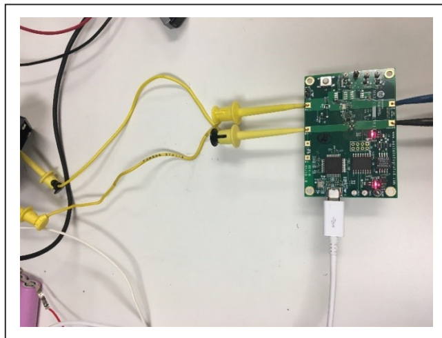
Figure 21. Bad Hardware Connection Example (Use power supply with lab jumper cable.)
