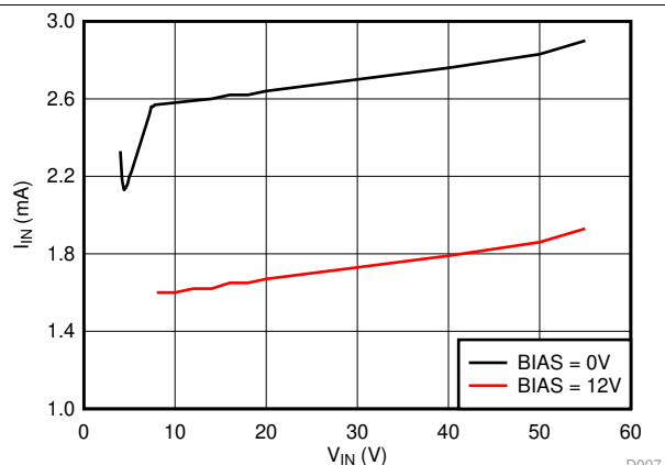
Figure 5. I_{IN} Operating vs V_{IN}
