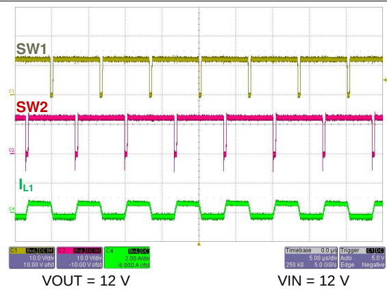
Figure 12. Forced CCM Operation (Buck-Boost)
