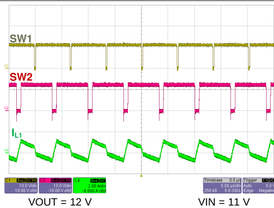
Figure 11. Forced CCM Operation (Buck-Boost)
