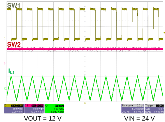
Figure 14. Forced CCM Operation (Buck)
