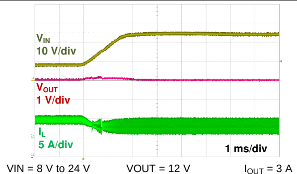
Figure 18. Line Transient
