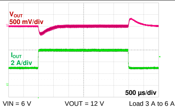
Figure 15. Load Step (Boost)
