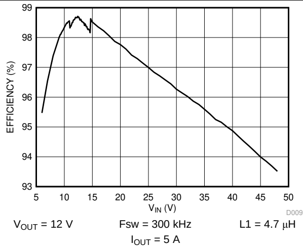
Figure 1. Efficiency vs V_{IN}
