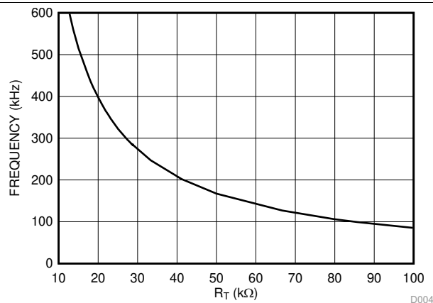
Figure 3. Oscillator Frequency
