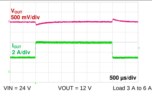
Figure 17. Load Step (Buck)
