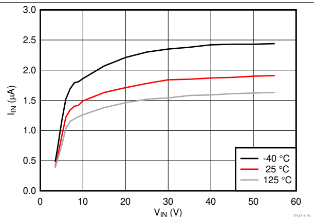
Figure 6. I_{IN} Shutdown vs V_{IN}
