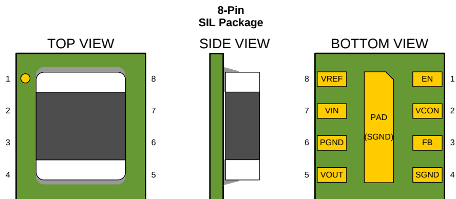
Pin Functions
