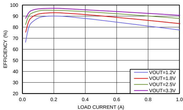
Typical Efficiency at V_{IN} = 3.6 V
