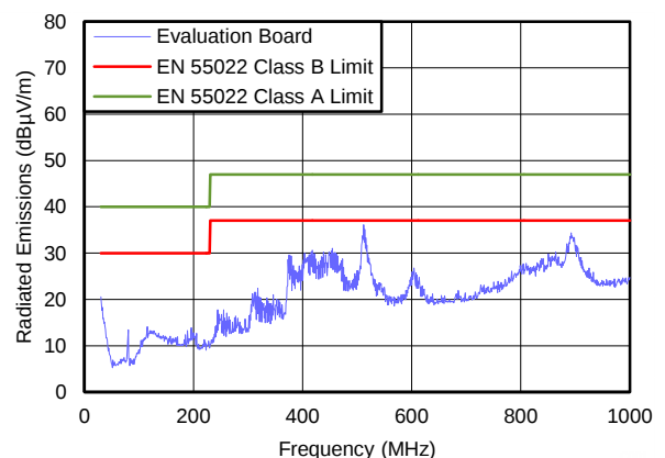
Radiated EMI (CISPR22) V_{IN} = 5 V, V_{OUT} = 1.8 V, I_{OUT} = 1 A
