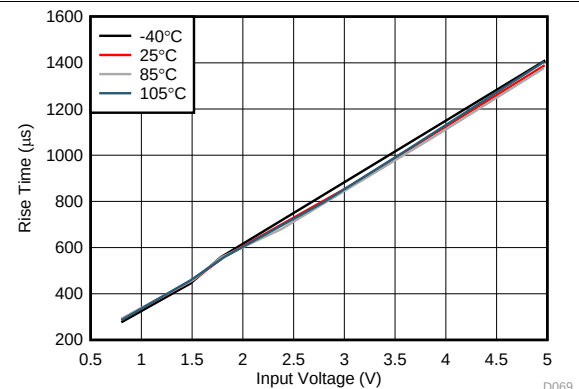
Figure 18. Input Voltage vs Turnon Time
