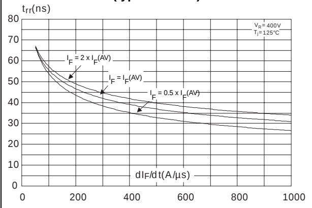
Figure 6: Reverse recovery time versus di/dt (typical values)
