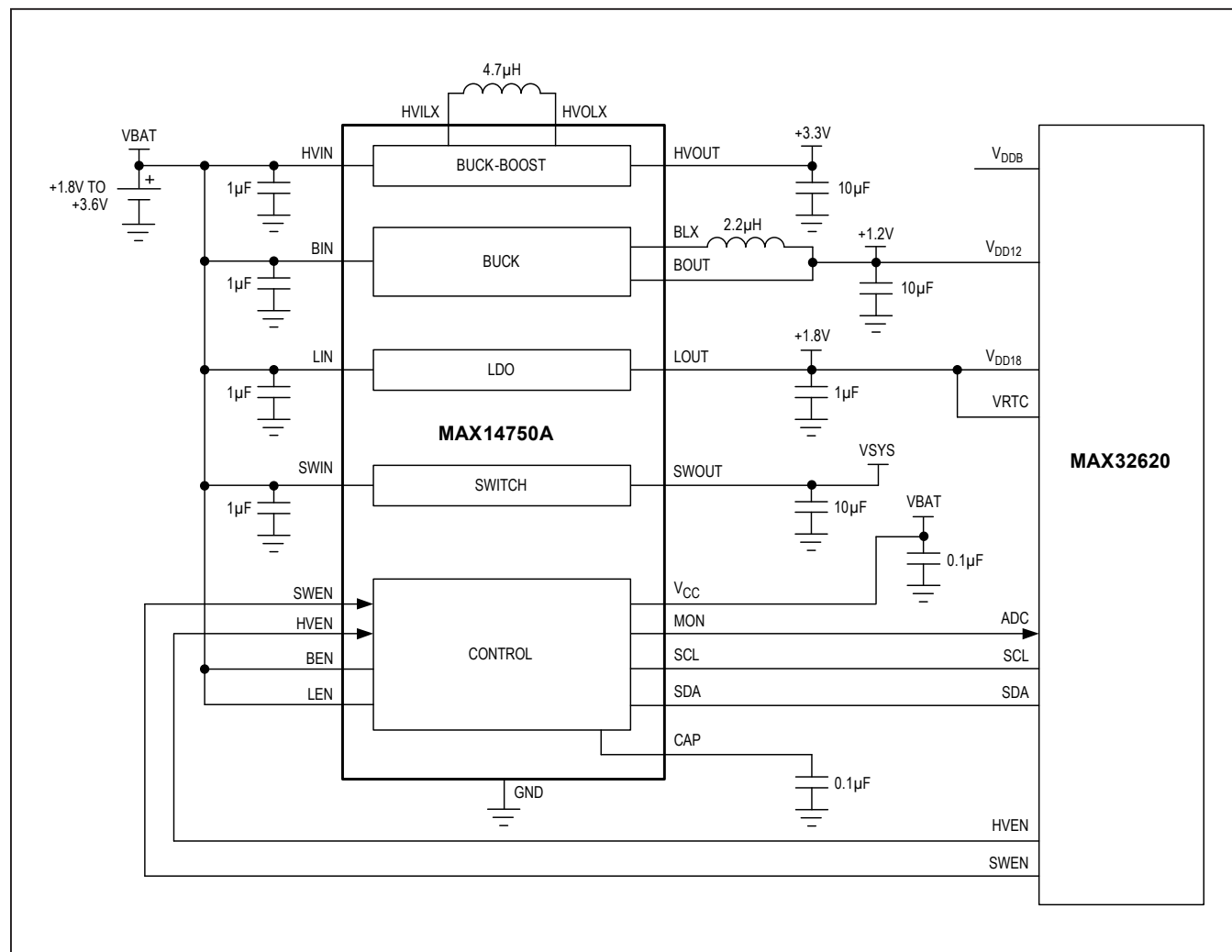
Figure 13. Always-On Coin Cell
