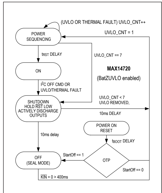
Figure 2. BatZUVLO enabled for MAX14720
