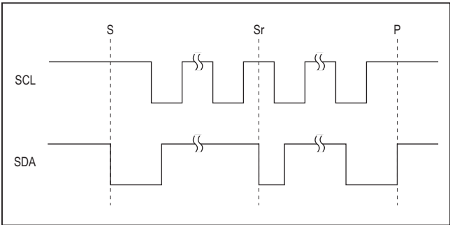
Figure 5. I2C START, STOP, and REPEATED START Conditions
