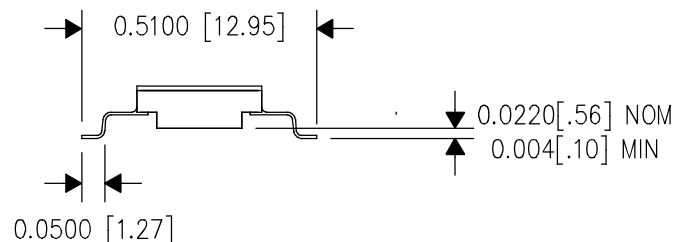
Figure 29. Typical HKU Package With Leads Form
