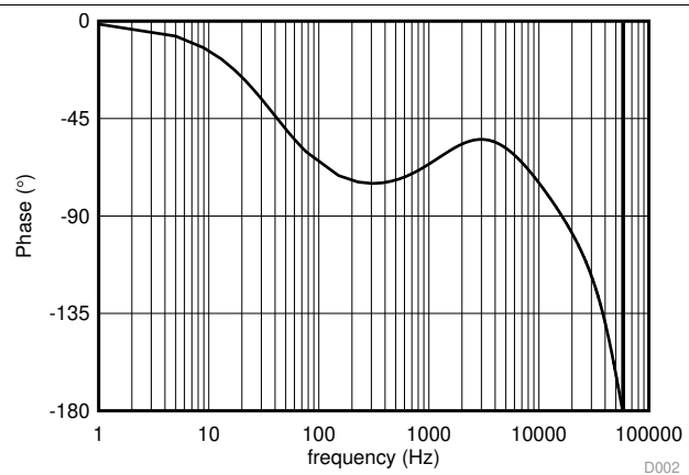
Figure 32. Converter Open-Loop Bode Plot - Phase
