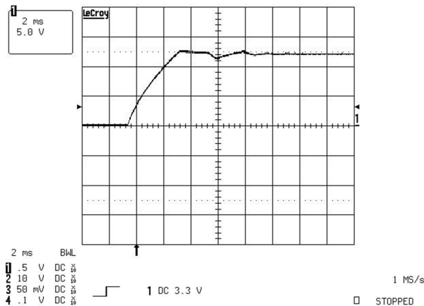
Figure 39. Output Voltage Behavior at Full Load Start-up (5 V/div)
