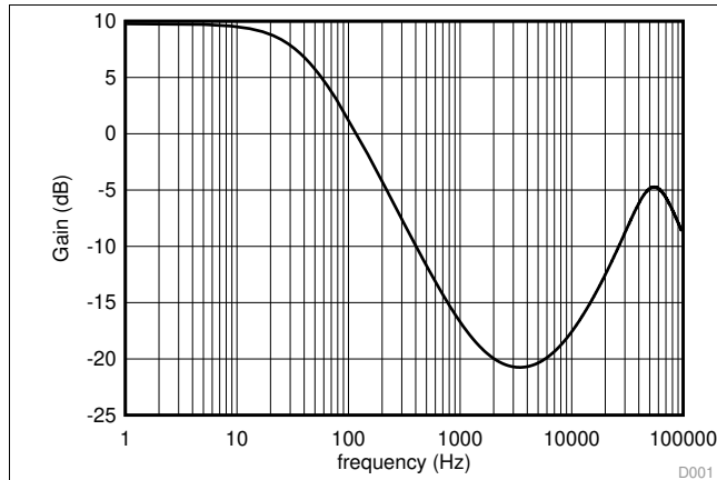
Figure 31. Converter Open-Loop Bode Plot - Gain
