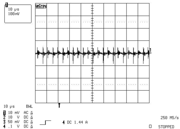
Figure 38. Output Voltage Ripple at Full Load (100 mV/div)
