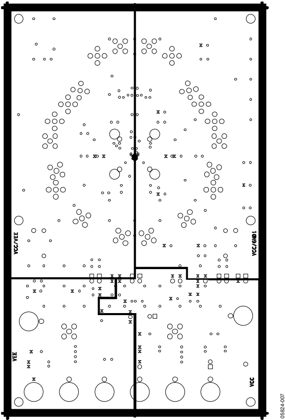
Figure 6. Buried Planes 1
