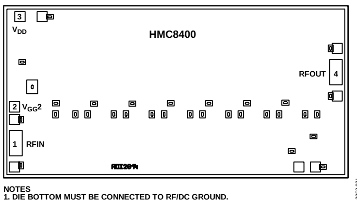
Figure 2. Pad Configuration
