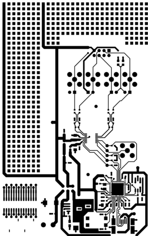
Figure 7. AD7797 Evaluation Board Component Side Artwork
