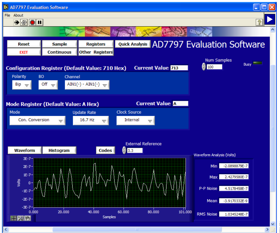
Figure 4. AD7797 Evaluation Software Registers Window
