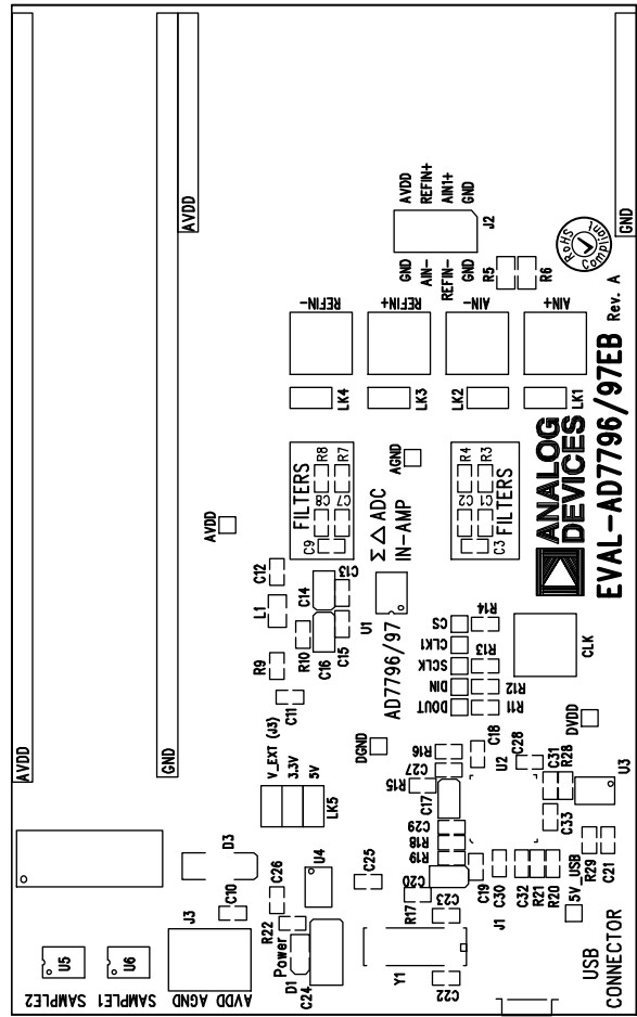
Figure 9. AD7797 Evaluation Board Component Layout Diagram
