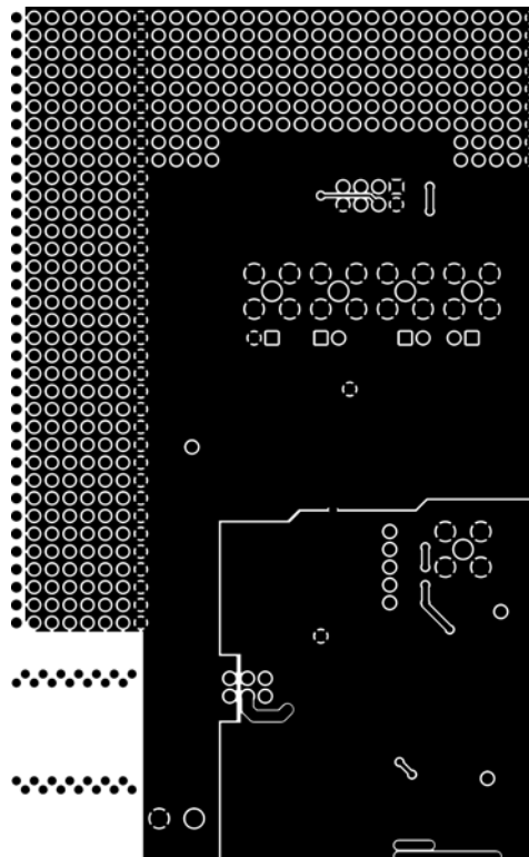
Figure 8. AD7797 Evaluation Board Solder Side Artwork
