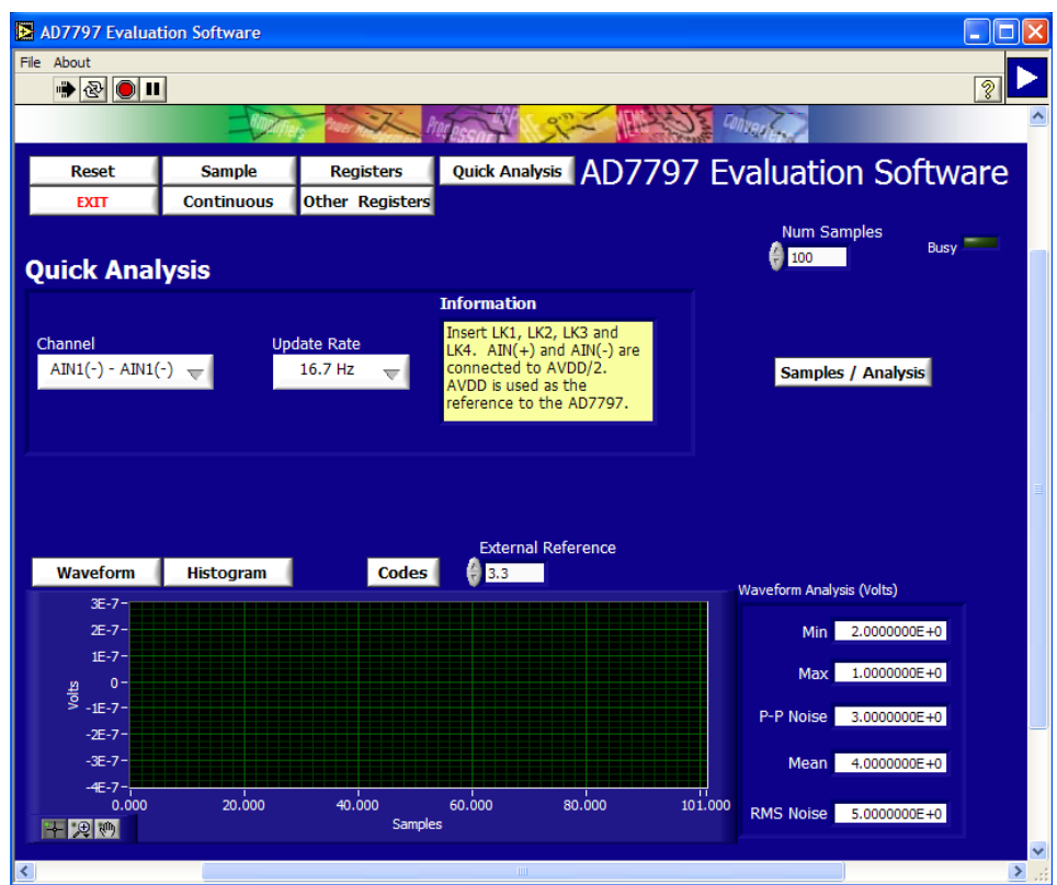
Figure 3. AD7797 Evaluation Software Main Window
