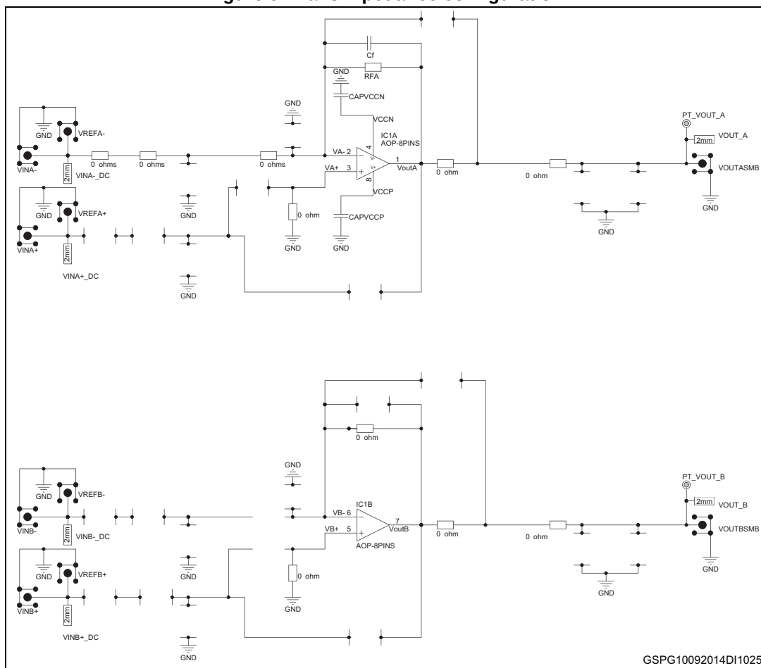
Figure 9. Transimpedance configuration
