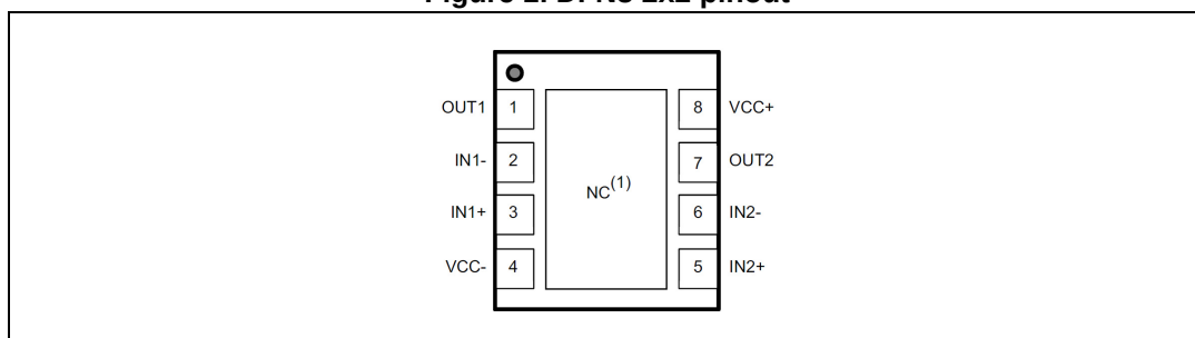
Figure 1. DFN8 2x2 pinout
