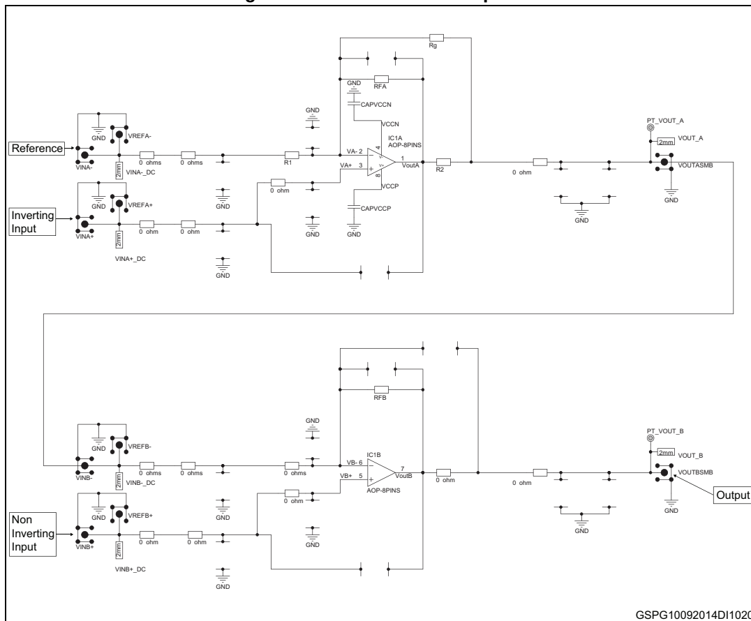
Figure 8. Instrumentation amplifier
