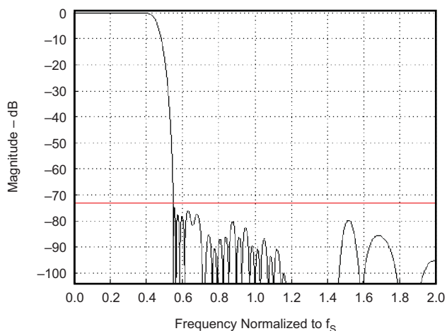
Figure 2-18. ADC Decimation Filter A, Frequency Response
