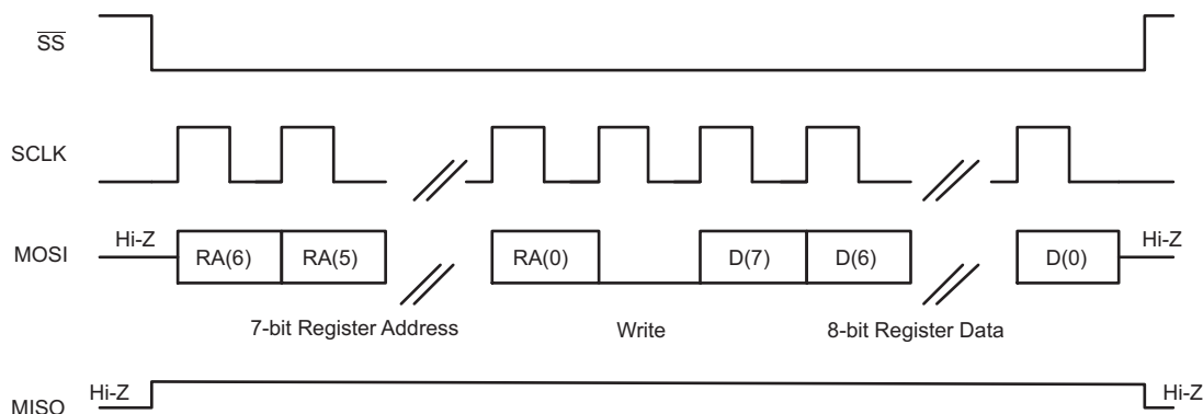
Figure 2-54. SPI Timing Diagram for Register Write
