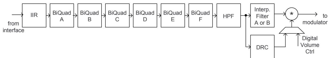
Figure 2-25. Signal Chain for PRB_P2, PRB_P5, PRB_P10 and PRB_P15
