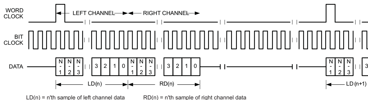
Figure 2-45. Timing Diagram for DSP Mode
