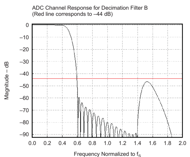
Figure 2-19. ADC Decimation Filter B, Frequency Response
