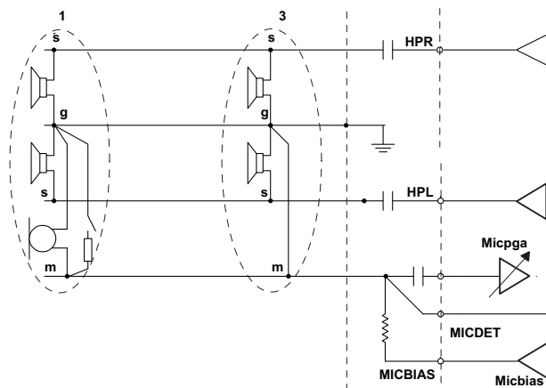
Figure 2-56. Jack Connections for Headset Detection
