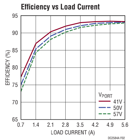
Figure 2. Efficiency (End-to-End)
