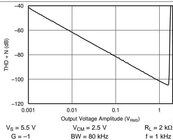
Figure 16. THD + N vs Amplitude
