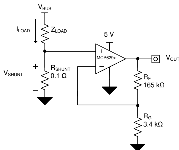
Figure 33. MCP629x in a Low-Side, Motor-Control Application
