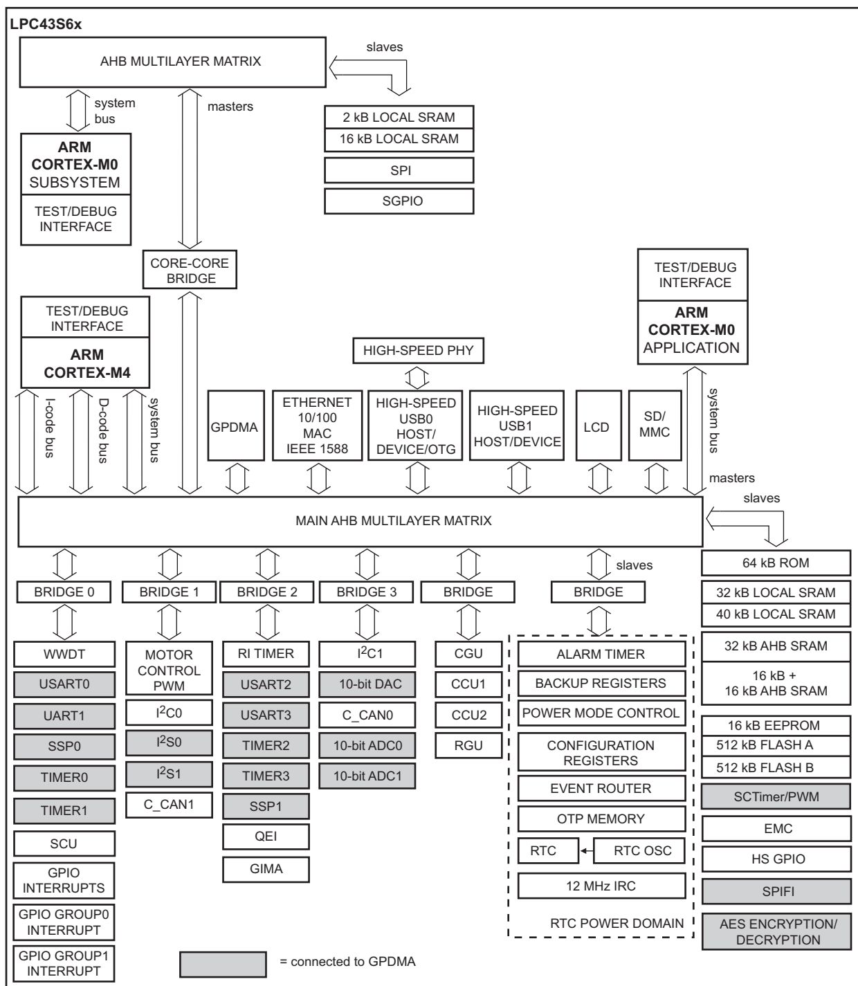
Fig 1. LPC43S6x Block diagram
