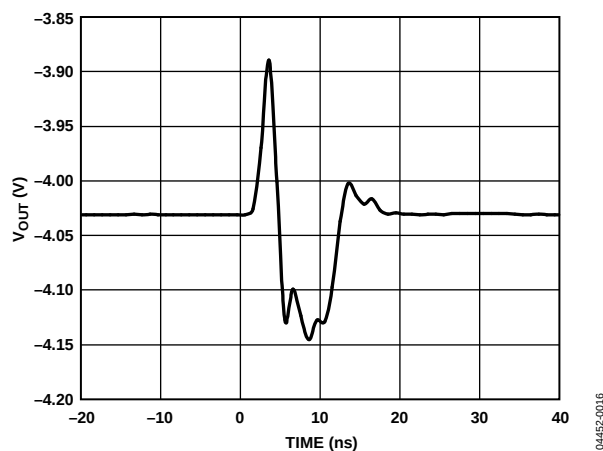
Figure 16. AD5547 Midscale Transition and Digital Feedthrough
