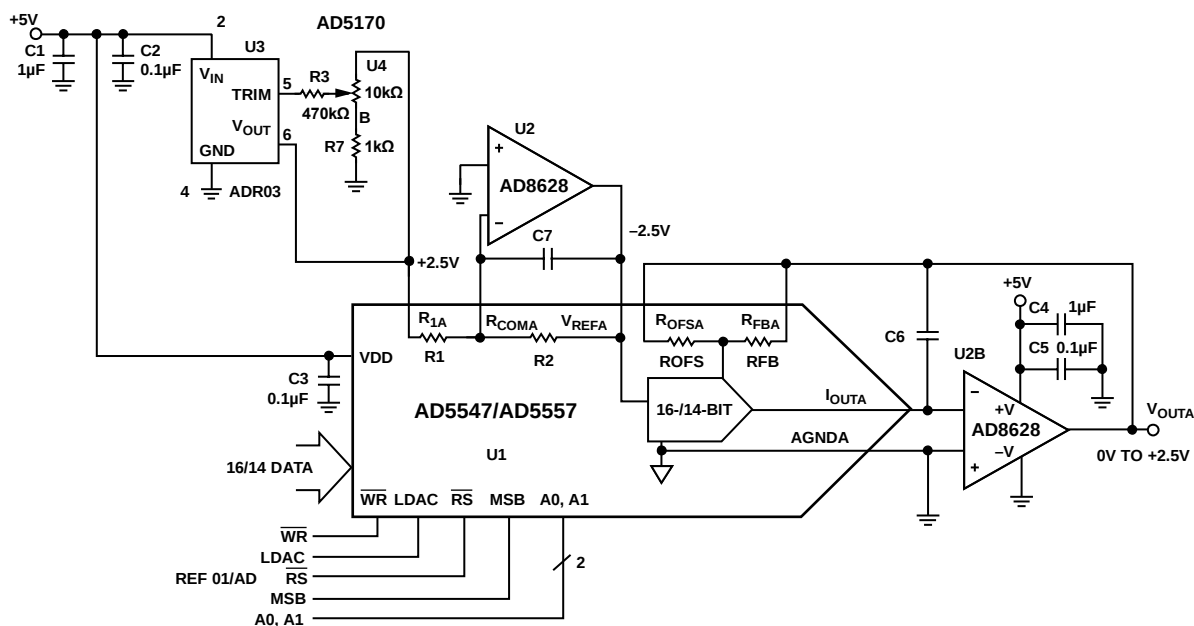
Figure 25. Full-Span Calibration
