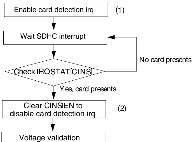
Figure 47-39. Flow diagram for card detection
