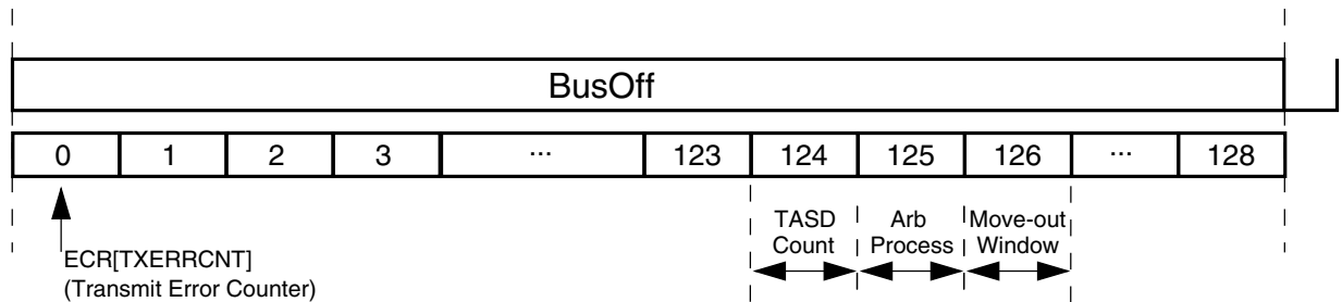
Figure 43-102. Arbitration at the end of bus off and move-out time windows
