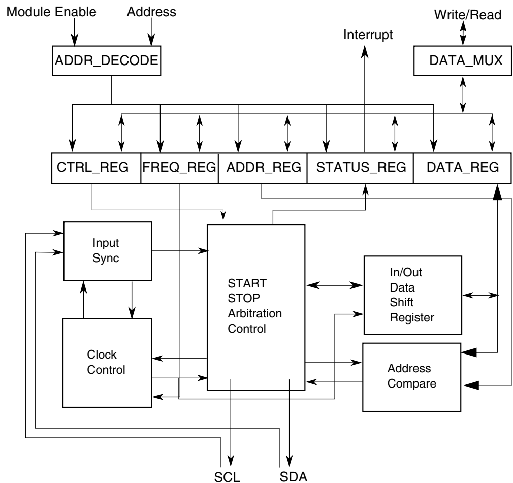
Figure 45-1. I2C Functional block diagram
