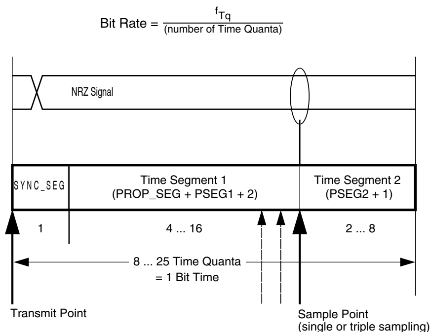
Figure 43-99. Segments within the bit time
