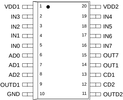
Figure 3. 33287 Pin Connections
