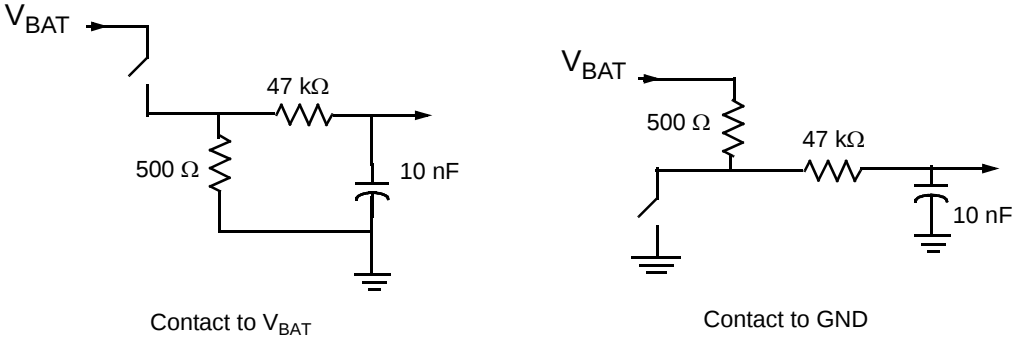
Figure 7. Contact Configuration
